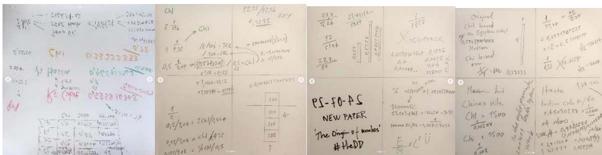
Notes originales Xi-quence CHI:Cubit ratio Double soleil 17.28 INV. Provient LI, CHI, Hasta
